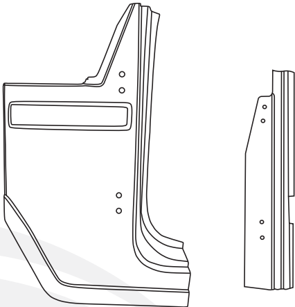
PM - 0257 Front Hawabari Assy.
