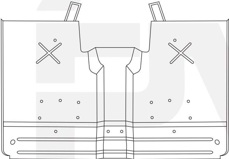
PM - 0305 Bol/Pickup Front Flooring Assy.
