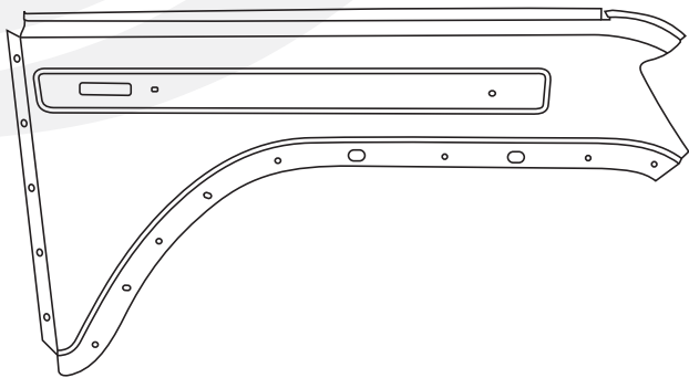
PM - 0011 Front Mudguard Cover T/2
