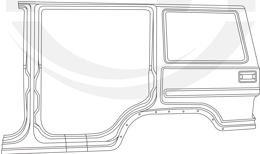
PM - 0068 Full Side Outer (Bol/Refresh)
