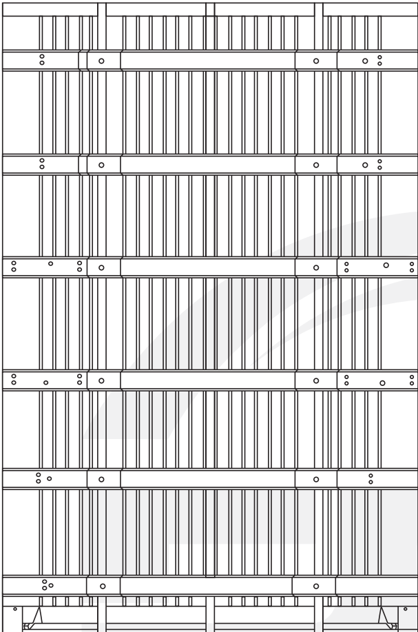
PM - 0633 Rear Flooring Assy.
