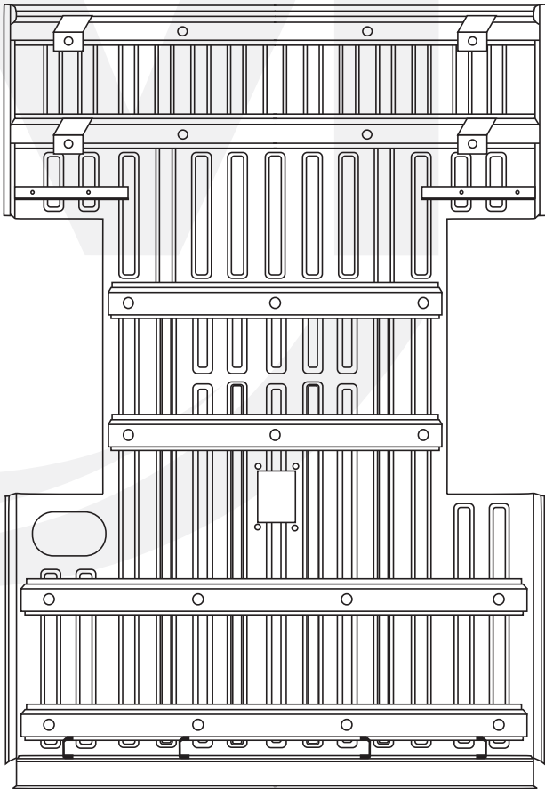
PM - 0564 Rear Dhala Flooring Assy.
