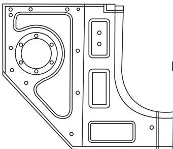
PM - 0039 Front Speaker Patra Inner
