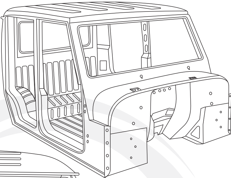
PM - 0521 Utility Body Assy. (Cabin)
