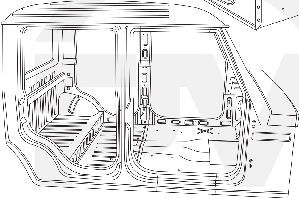
PM - 0522 Body Assy. T/1 (Cabin)
